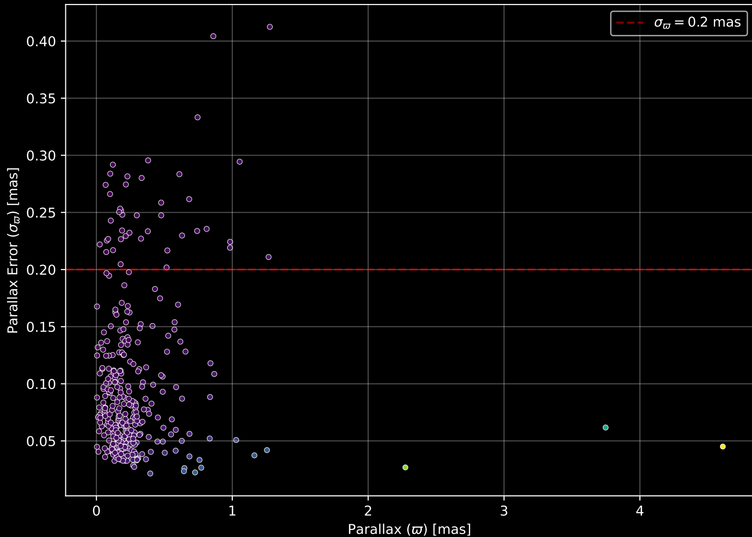
APOGEE DR17 Field: [003-02-O] Parallax Quality (n= 333)
