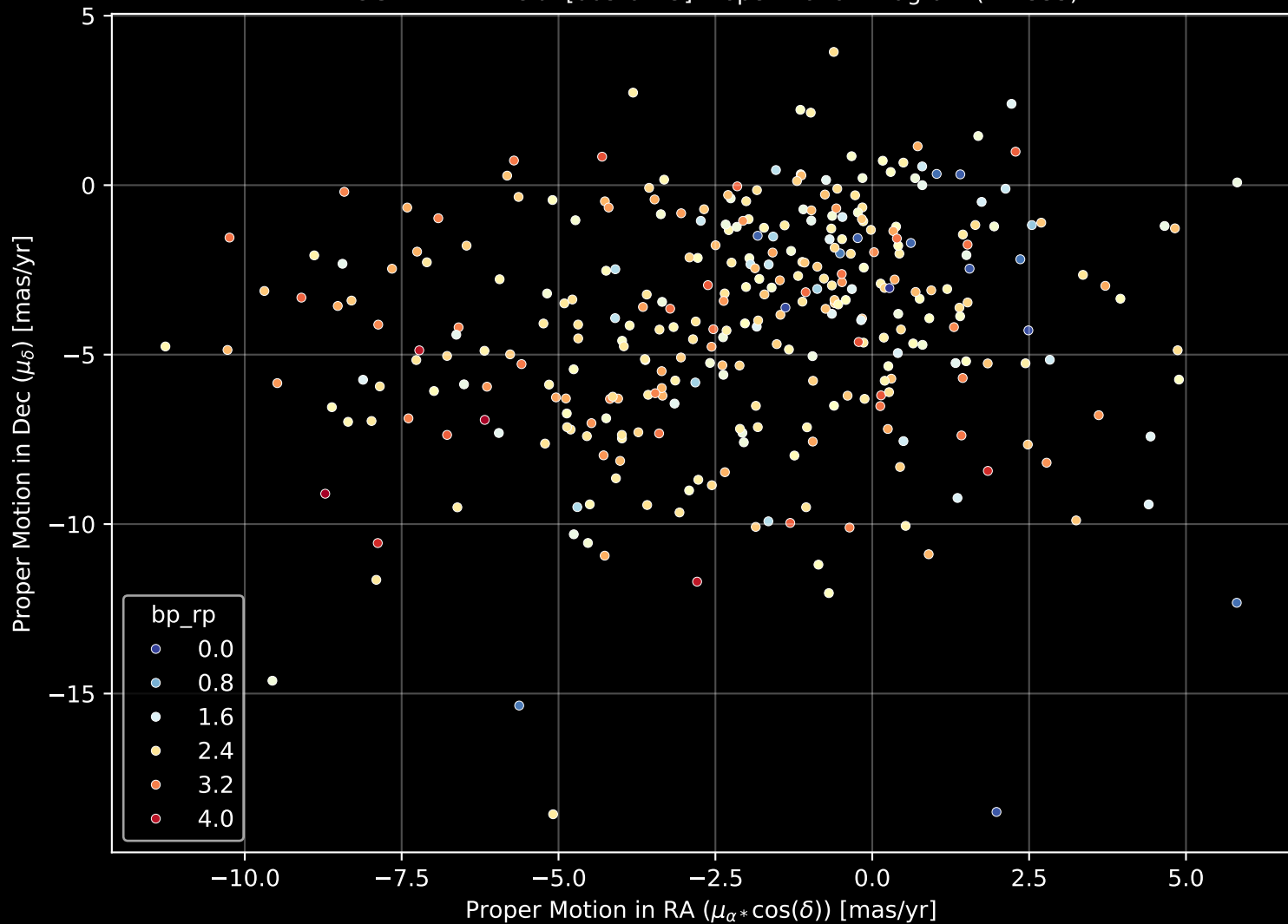
APOGEE DR17 Field: [003-02-O] Proper Motion Diagram (n= 333)
