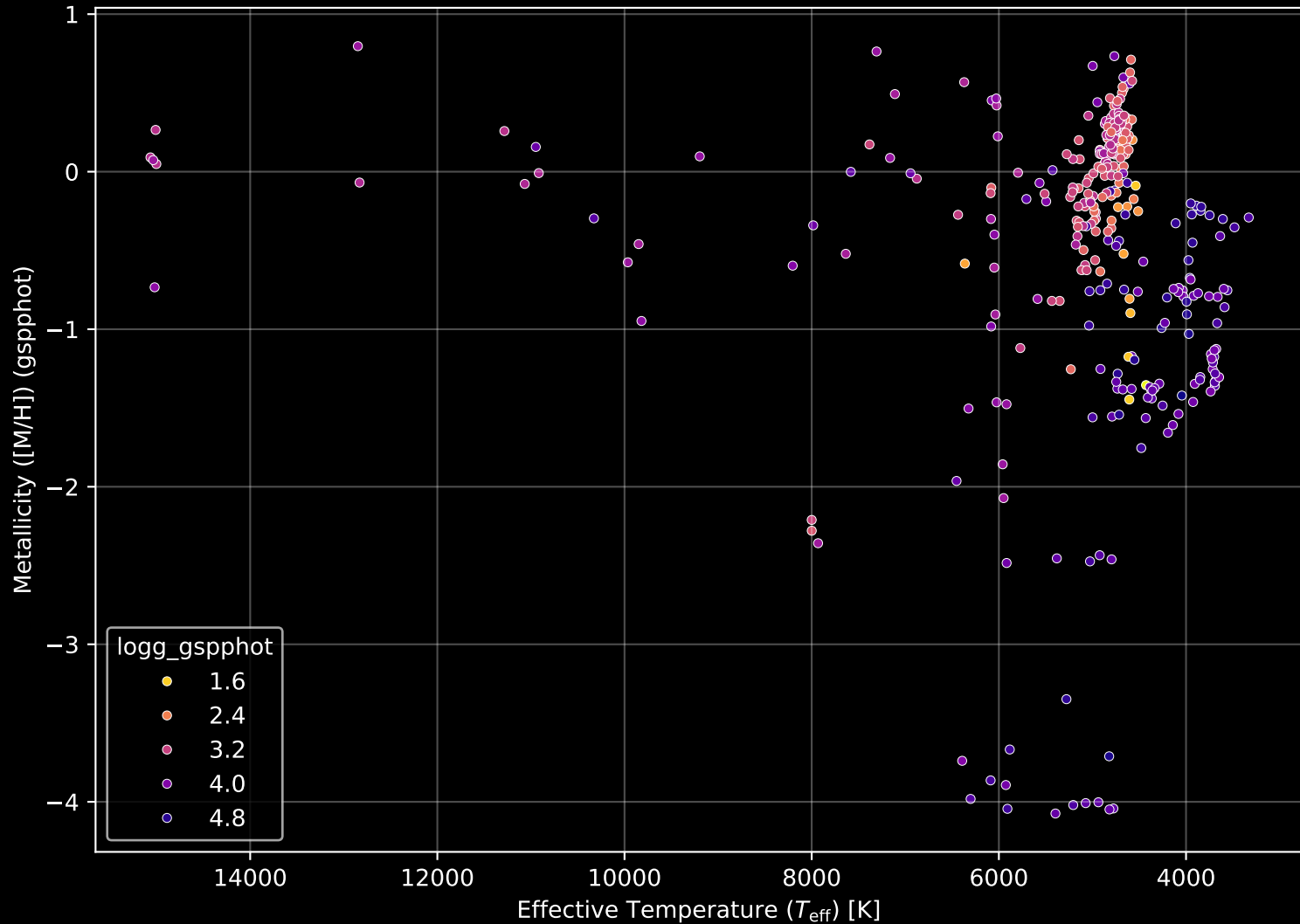
APOGEE DR17 Field: [003-02-O] Stellar Population Parameters (n= 333)
