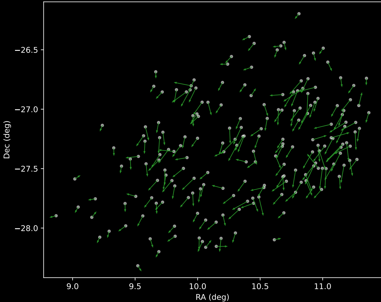
APOGEE DR17 Cluster 4 Proper Motion Vectors (n=191)
