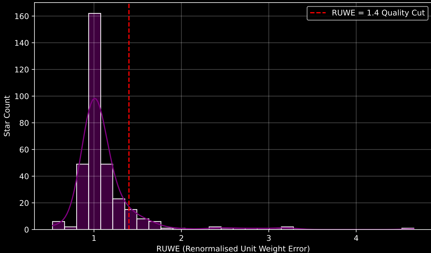
GAPOGEE DR17 Field [003-02-O] RUWE Distribution (n= 332)
