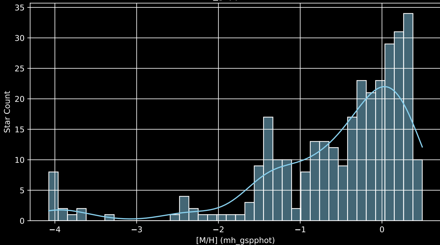
APOGEE DR17 Field: [003-02-O] [M/H] (mh_gspphot) (n= 320)
